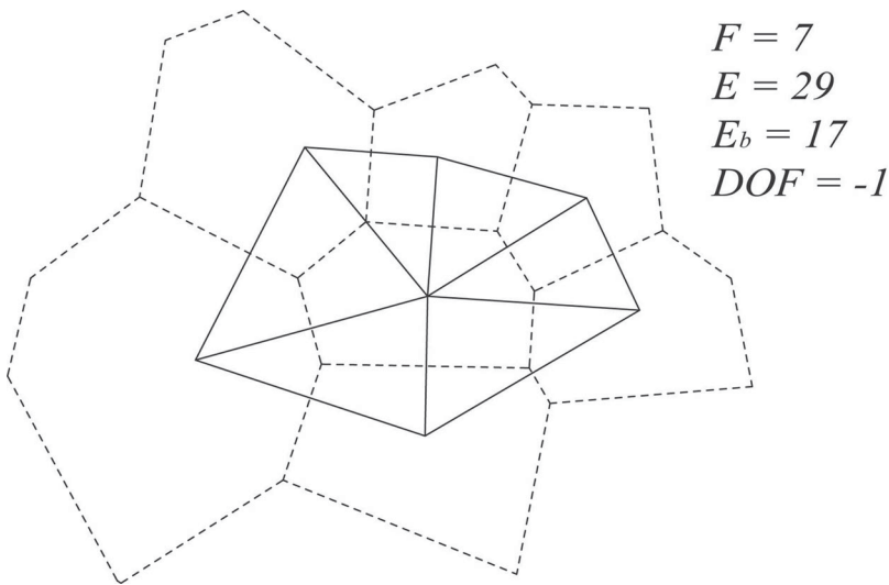
Figure 16. A Voronoi diagram and its dual.
